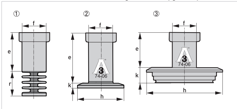
Figure 6-3: Dimensions for pressure transmitter with cooling fins and hygienic process connections
