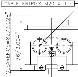
FLAT ALUMINUM OR RESIN COVER WITH ARROW INDICATOR
