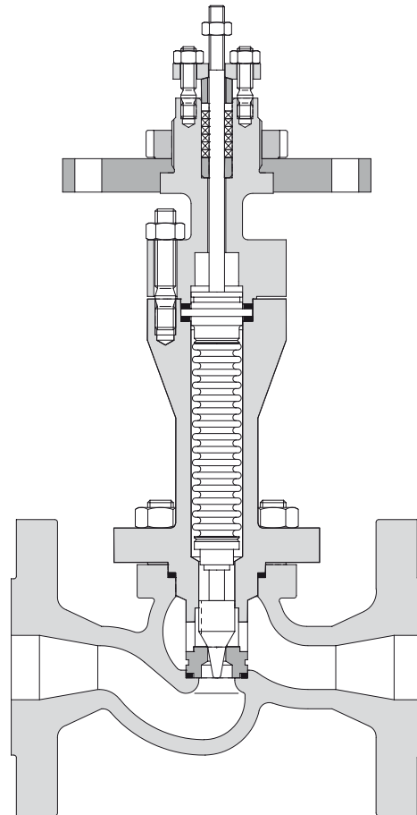
Bellows Seal
