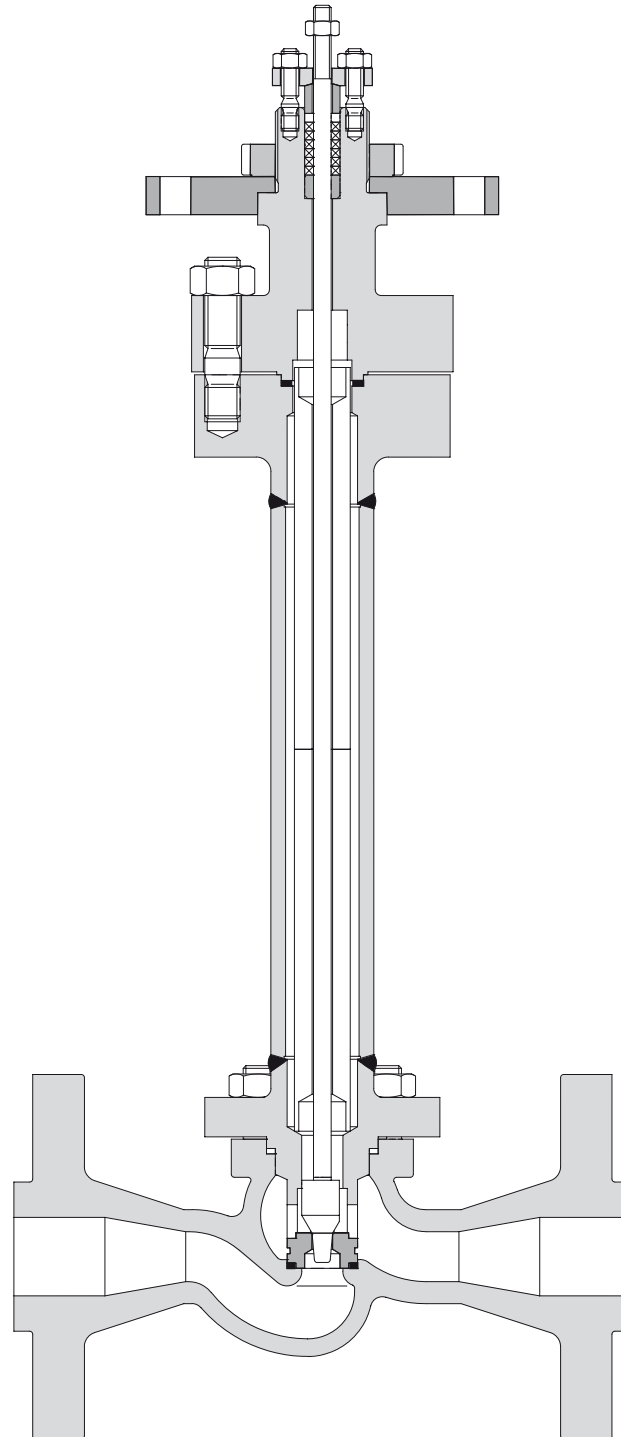
Cryogenic Extension
