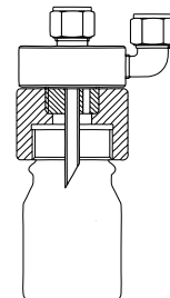
Type B with PTFE-adaptor for laboratory-bottle
