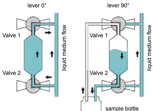
Type B with PTFE-adaptor for laboratory-bottle
